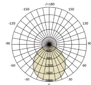
2X4 - 45W - RA80 - 4000K
